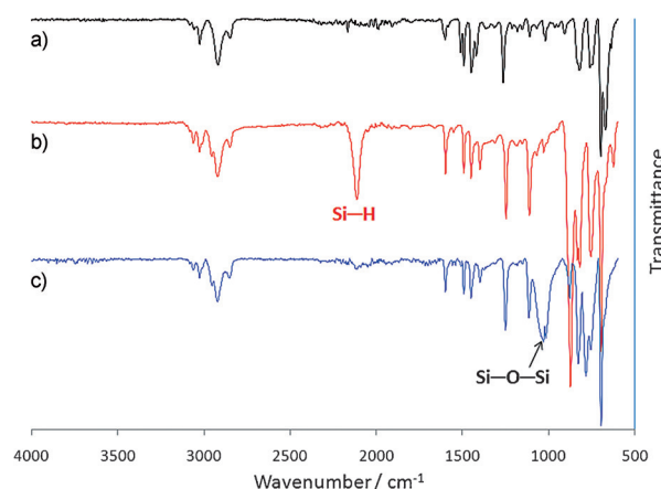
Figure 1. ATR-IR spectra of 4-bromopolystyrene bead (a), dimethylphenylsilane-derivatized polymer bead (b), and polymer bead after ozonization, MTO-catalyzed release of HOOOH and its removal from the solution (c).
