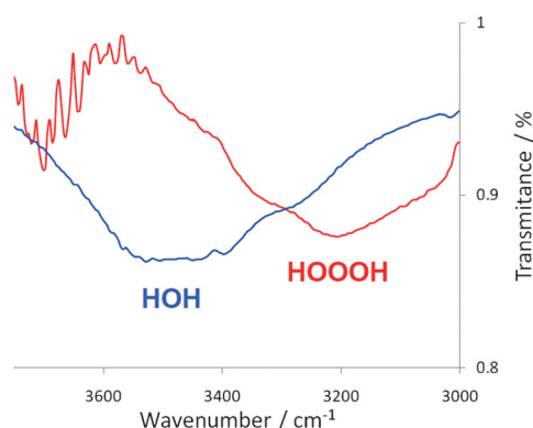
Figure 3. Sections of the low-temperature ATR-IR spectra of \text{HOOH} and \text{HOH} (for comparison) in acetone at -40^{\circ}\text{C} . See also the Supporting Information.
